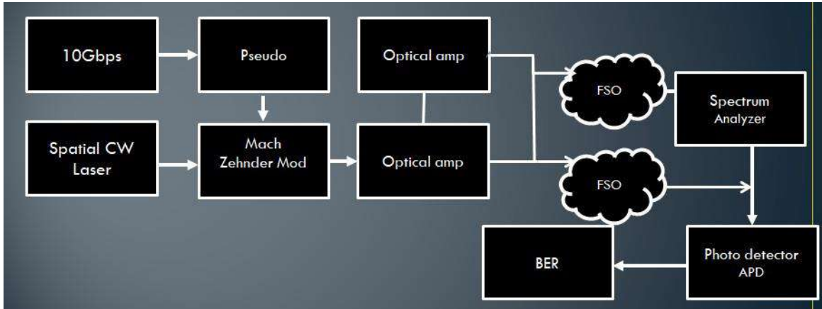
Figure 3.1: Proposed system with space & amplifier
