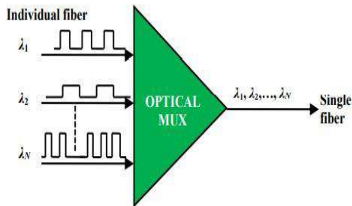
Figure 2.7: Basic building block of optical DWDM transmission
