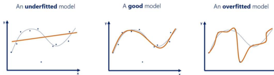
Figure: Understanding model via fit curve [37].
