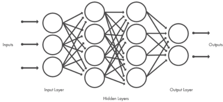
Figure: Layers of linked nodes make up neural networks. Hundreds of hidden layers may be found in networks.
