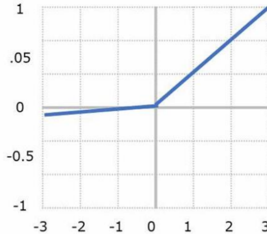
Figure: Leaky ReLU Function
