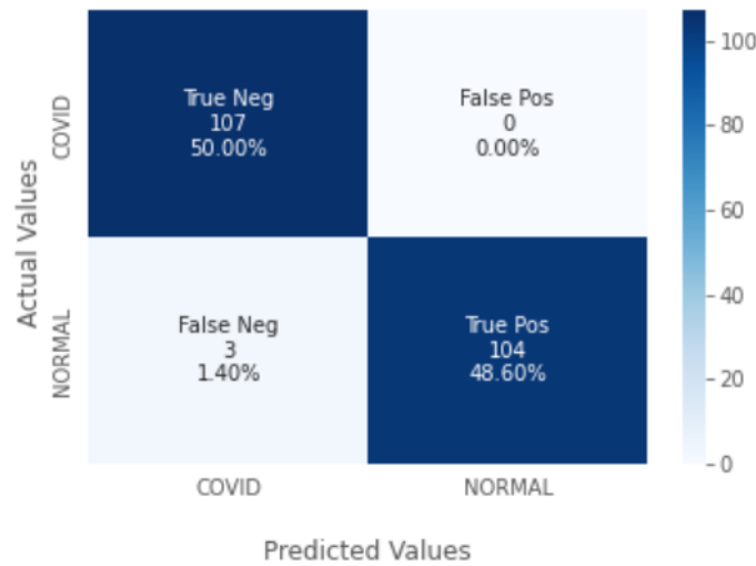
Figure: Confusion Matrix for the proposed model
