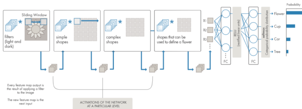
Figure: Different resolutions of filters are applied to each training picture, and the result of each convolved image serves as the input to the next layer.
