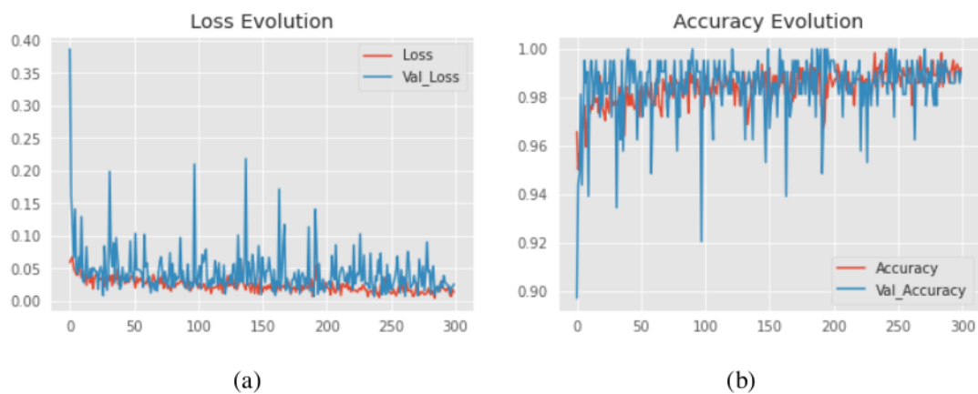
64 Figure: (a) Train and Validation loss vs. Epochs (b) Train and Validation accuracy vs. Epochs for the proposed COVID-Deep CNN.
