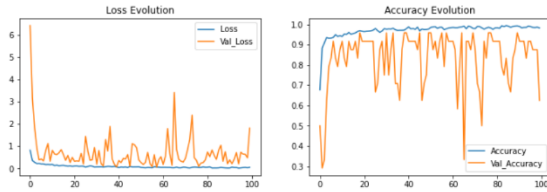
Figure: Accuracy and loss graph vs epochs of Inceptionv3 model
