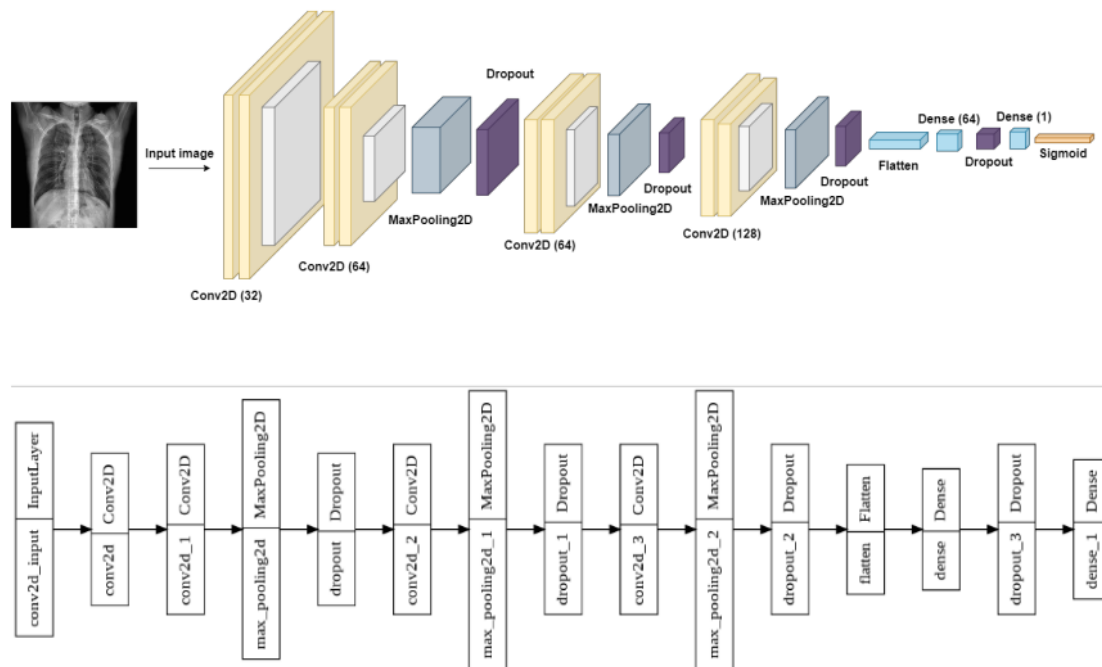
Figure: Proposed custom Convolutional Neural Network model layers
