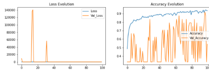
Figure: Accuracy and loss graph vs epochs of VGG16 model
