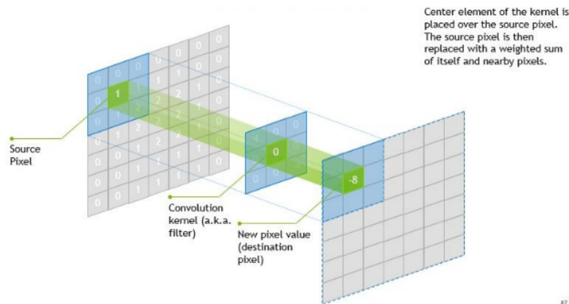
Figure: Convolutional layer [35]
