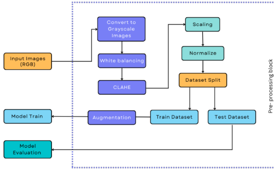
Figure: Preprocessing technique for our work in the diagram
