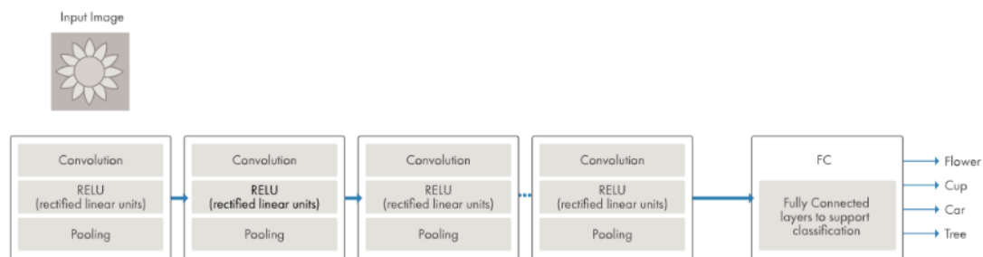
Figure: Illustration of a network with several convolutional layers
