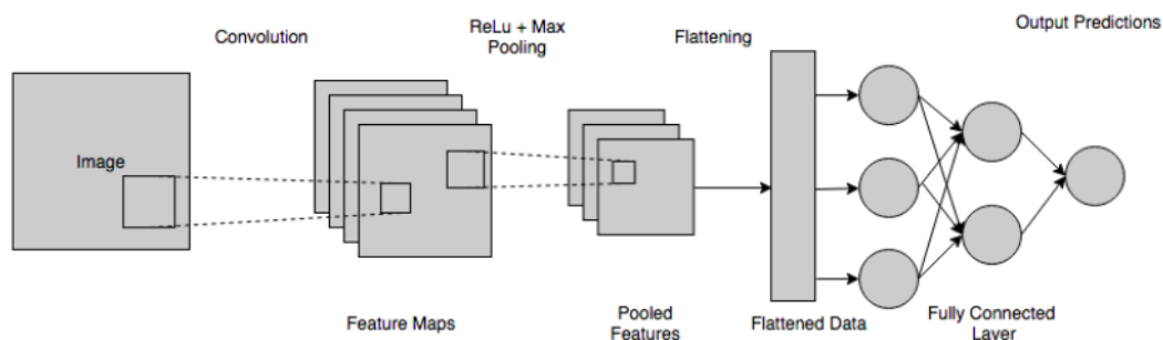
Figure: Layers of CNN
