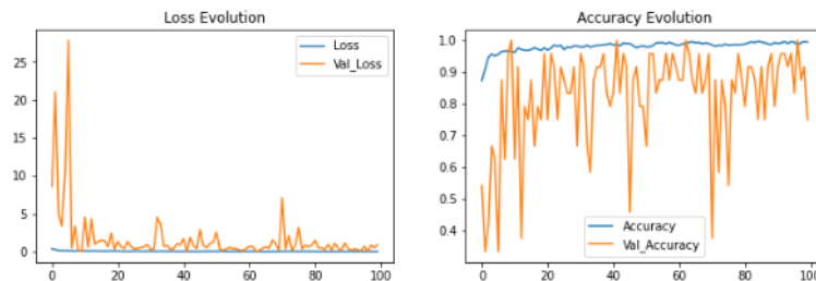
Figure: Accuracy and loss graph vs epochs of Densenet model
