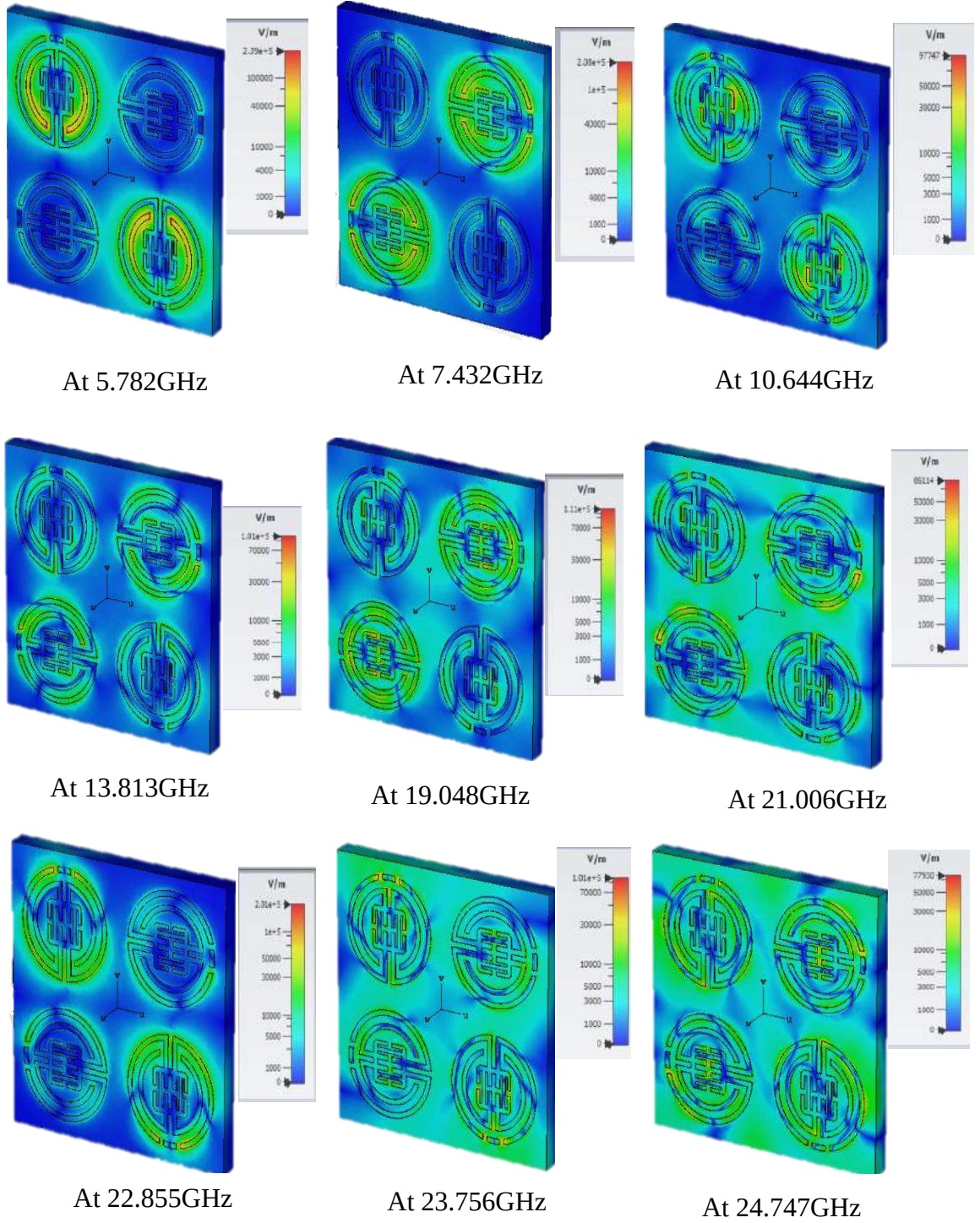
Figure 4.10: E-field for respectively 5.782 GHz, 7.432 GHz, 10.644 GHz, 13.813 GHz, 19.048 GHz, 21.006 GHz, 22.856 GHz, 23.756 GHz, and 24.746 GHz.
