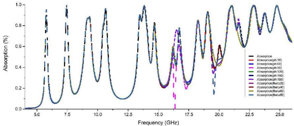
Figure 4.5: Polarization Insensitivity
