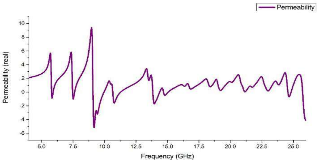
Figure 4.7: Permeability(real)
