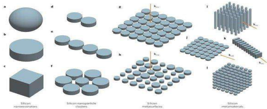
Figure 1.1: Metamaterials [2]
