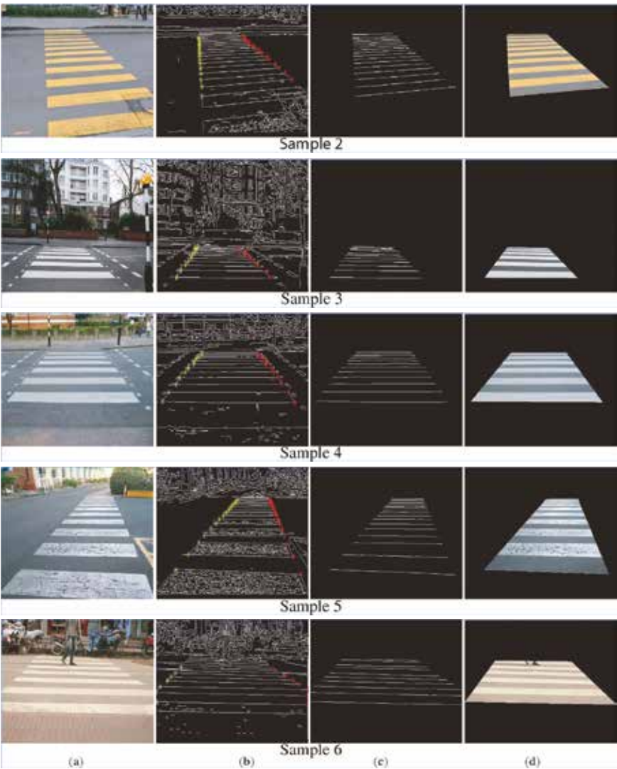
Figure 12 Processing example of pedestrian crossing region detection: a) input pedestrian crossing image, b) 2CP in edge image, c) arranging HEs in increasing sorted order, and d) detecting pedestrian crossing region
