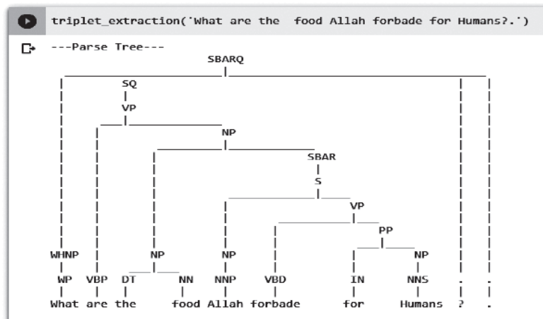
Fig 2: Generating Parse Trees from User Query by Using Stanford CoreNLP Parser
