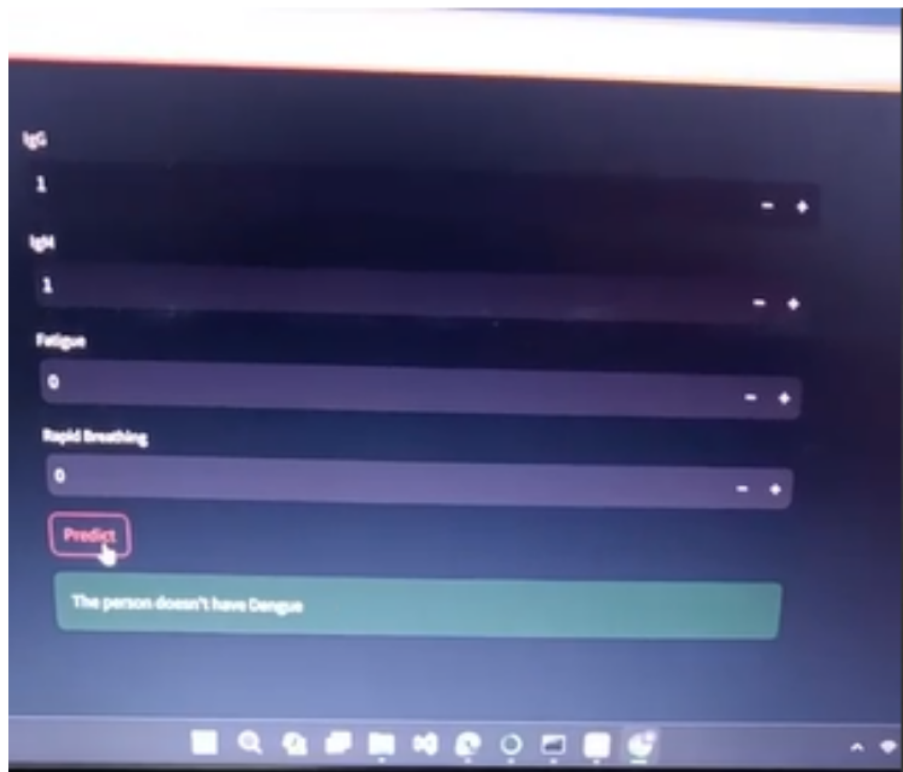
Fig. 4.20. Screenshot 3
