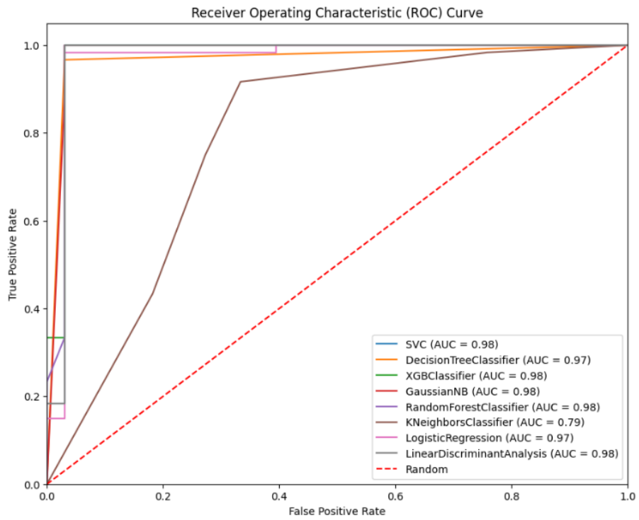
Fig. 4.16. ROC Curve
