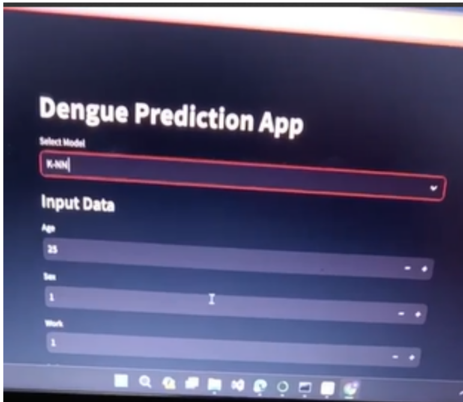
Fig. 4.18. Screenshot 1
