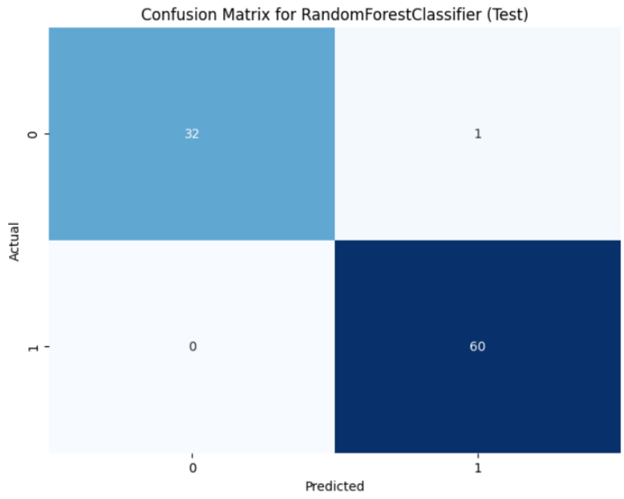
Fig. 4.15. Confusion Matrix for Random Forest
