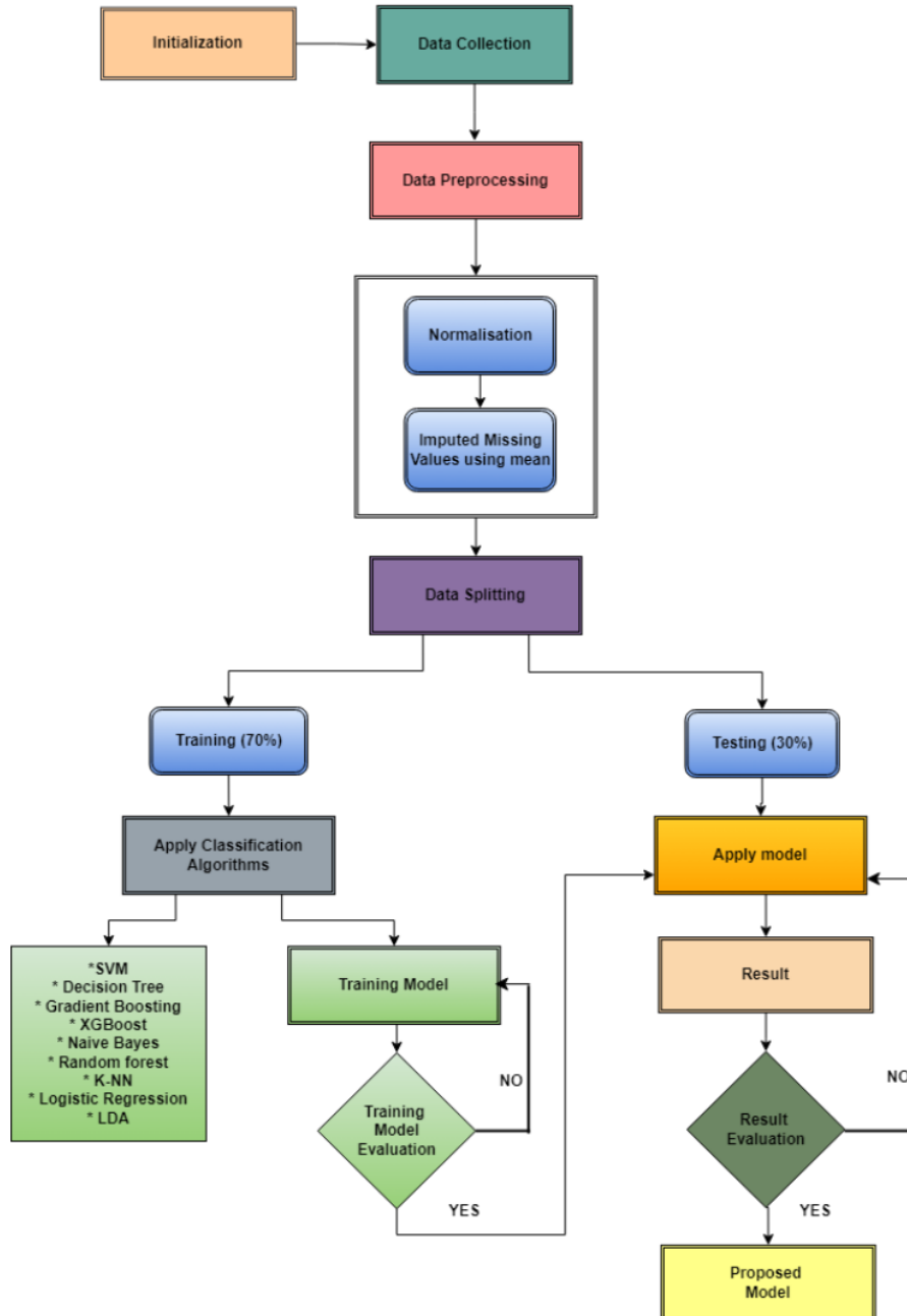
Fig. 3.1. Schematic diagram of Dengue prediction model
