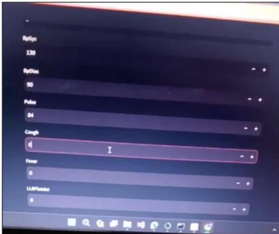
Fig. 4.19. Screenshot 2
