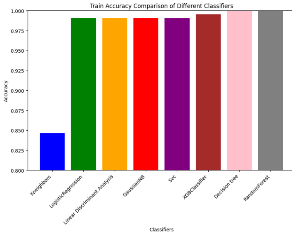
Fig. 4.12. Training Accuracy Comparison of different classifiers
