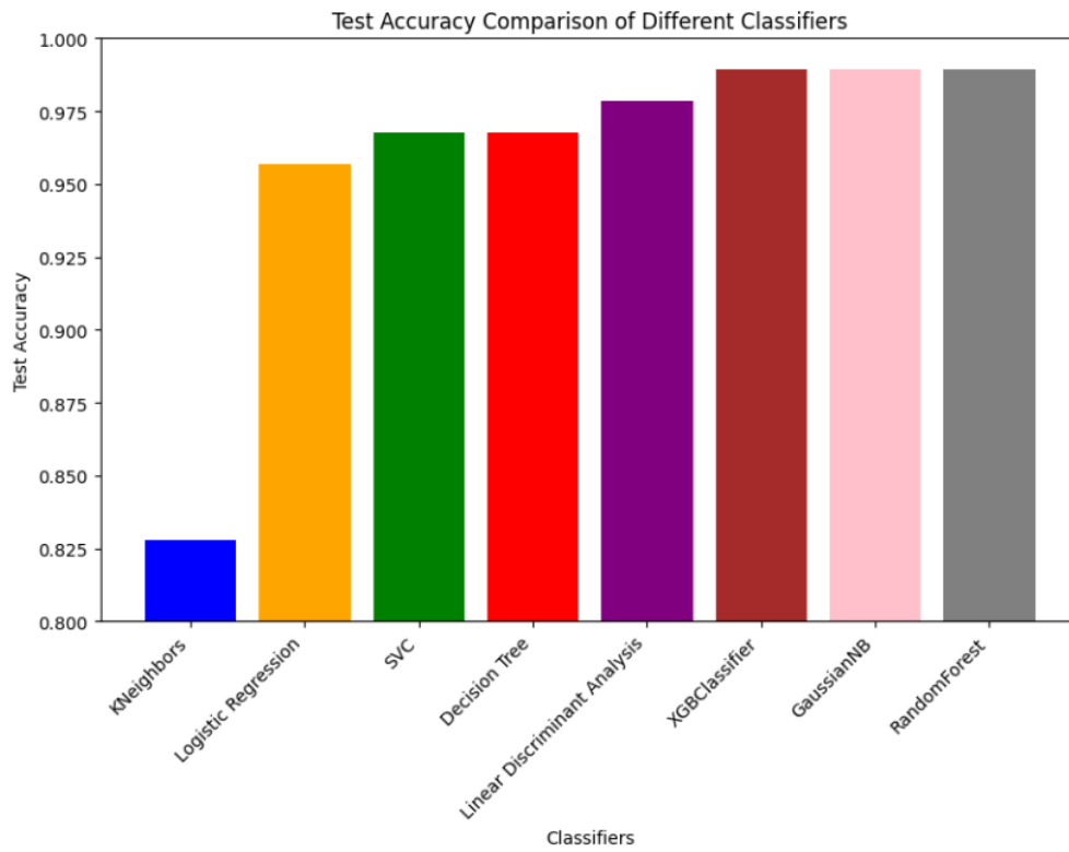
Fig. 4.13. Test Accuracy Comparison of different classifiers
