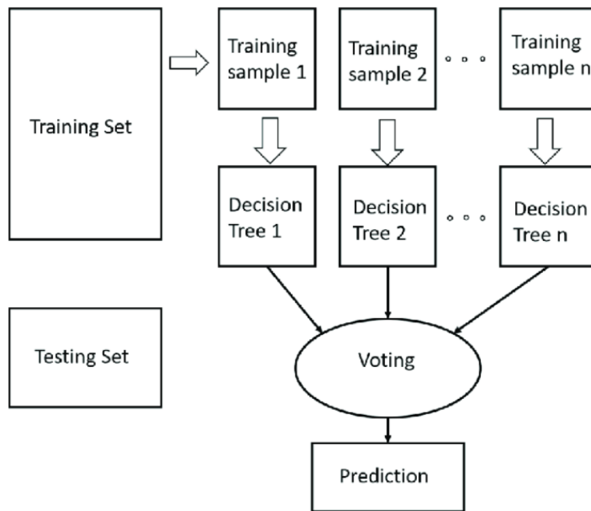
Fig. 3.2. The architecture of the Random Forest Classifier [21]
