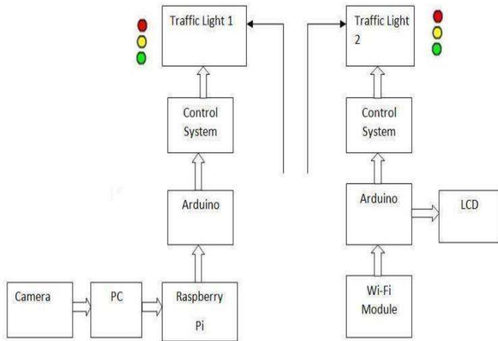
Fig 2.3 : Work Flow of Proposed Method
