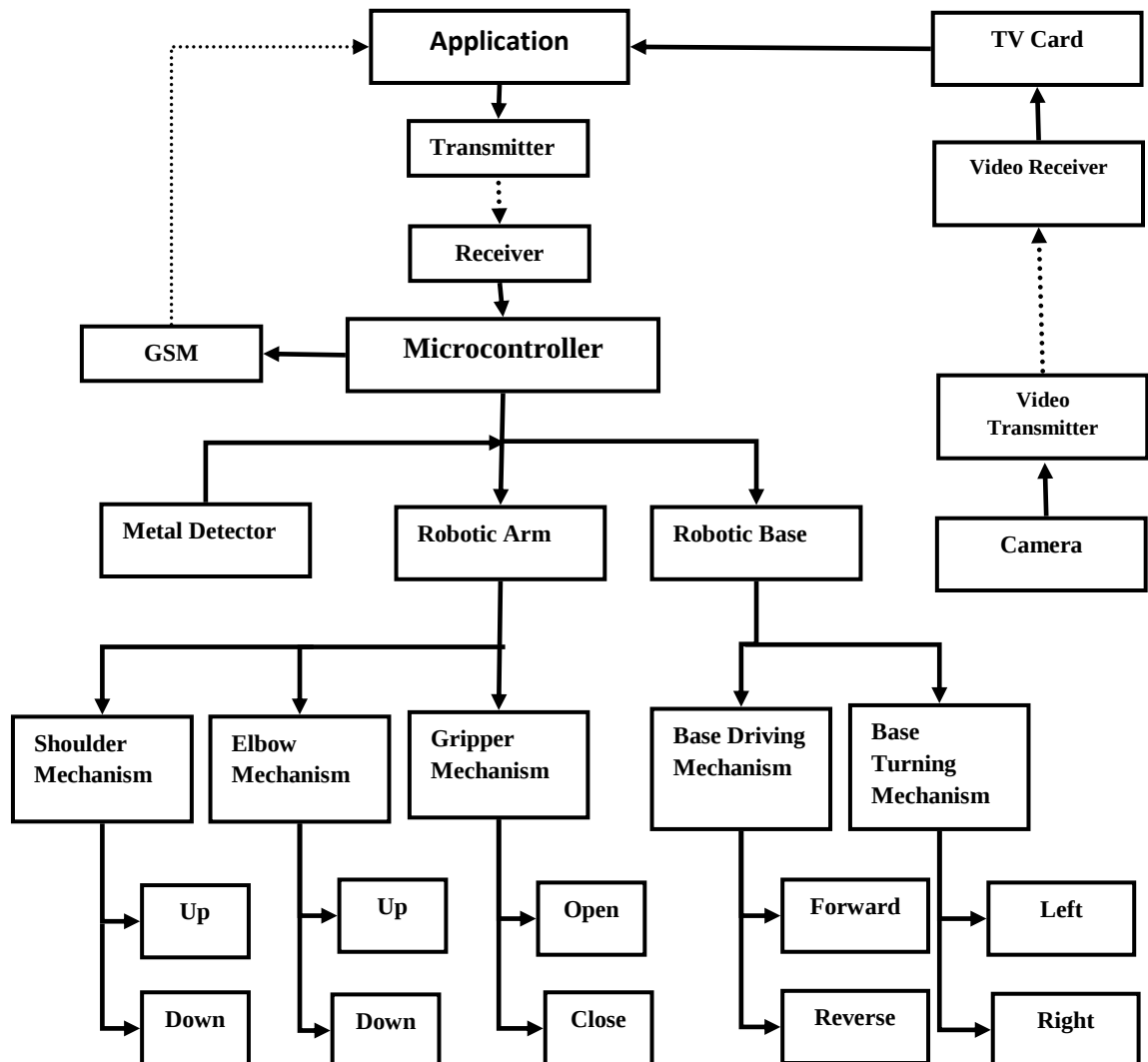
Fig. 5.1 system Architecture
