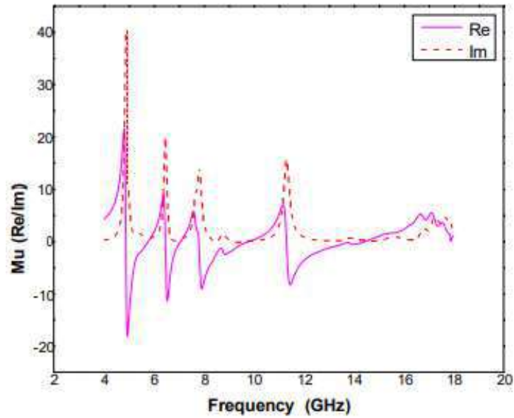
Figure 9 Permeability (Re/Im)
