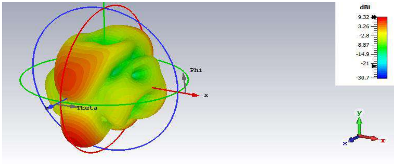
Figure 5.13: 3D Radiation Pattern of 1×4 array antenna at 28.3 GHz
