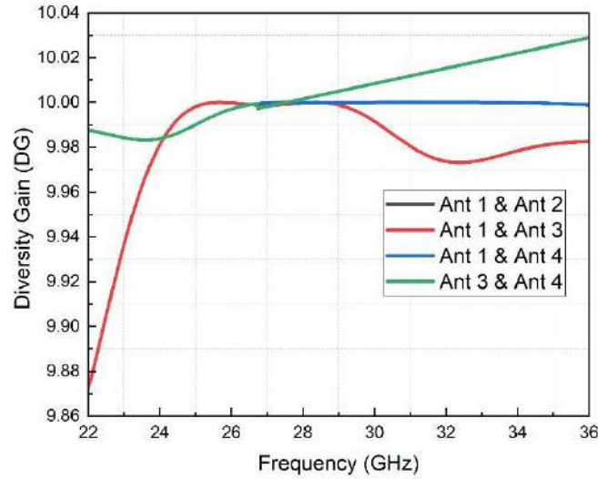
Figure 5.9: Diversity Gain of MIMO Antenna
