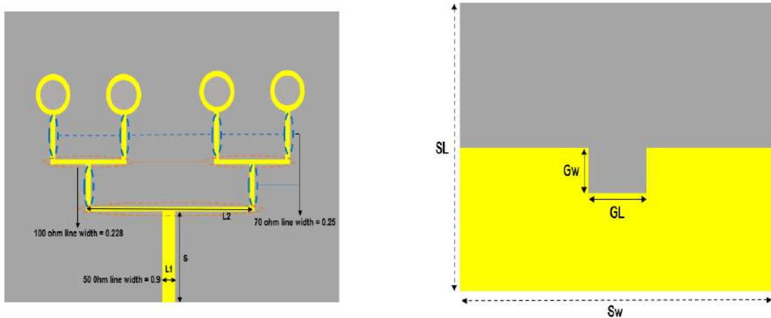
Figure 4.4: Structure of 1×4 Array Antenna with ground structure
