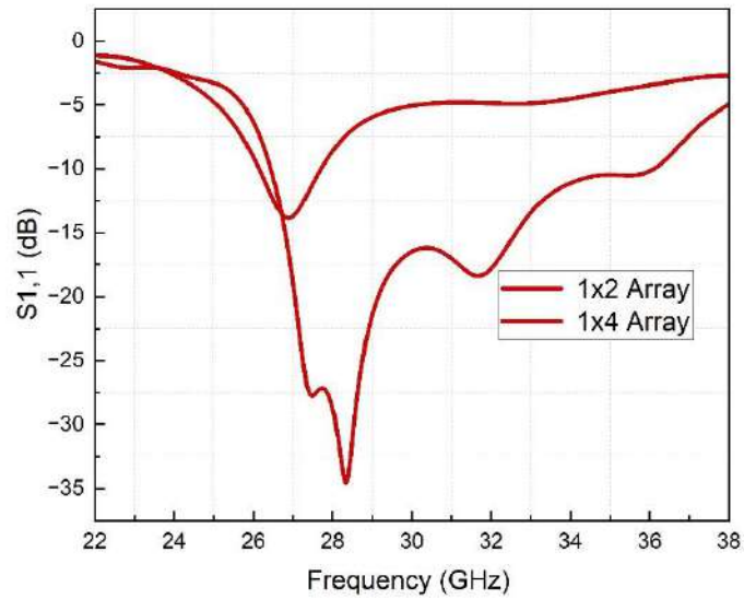
Figure 5.10: Return Loss Plot of 1x4 Array Antenna
