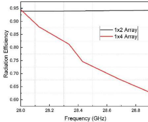
Figure 5.15: Radiation Efficiency of 1x4 Array Antenna
