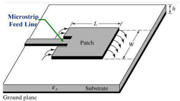
Figure 2.2: Microstrip Line Feeding Schematic
