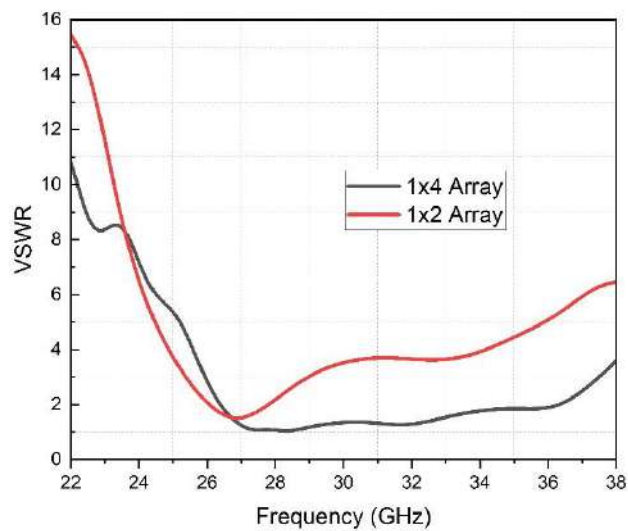
Figure 5.11: VSWR Plot of 1x4 Array Antenna
