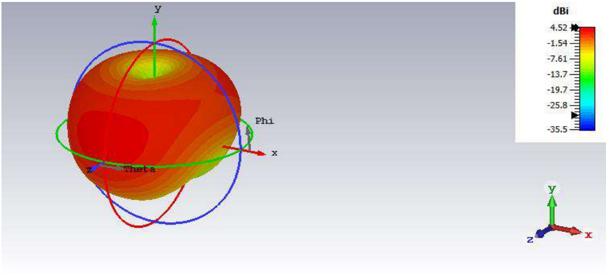
Figure 5.4: 3D Radiation Pattern of Single Element Antenna at 28 GHz
