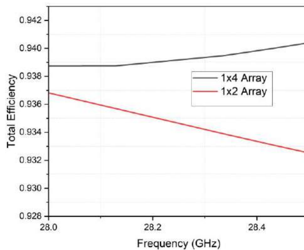
Figure 5.14: Antenna Efficiency of 1x4 Array Antenna
