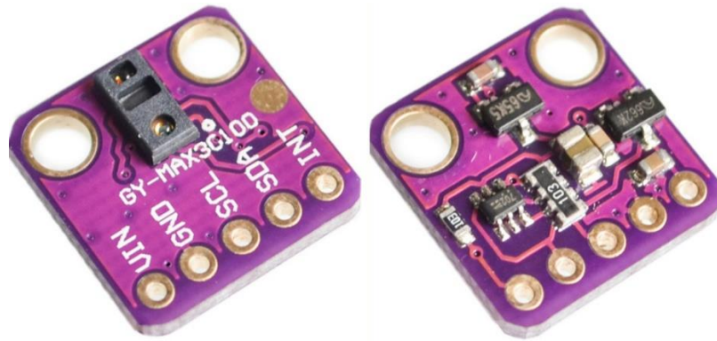
Figure 8 GY-MAX30100 [30]
