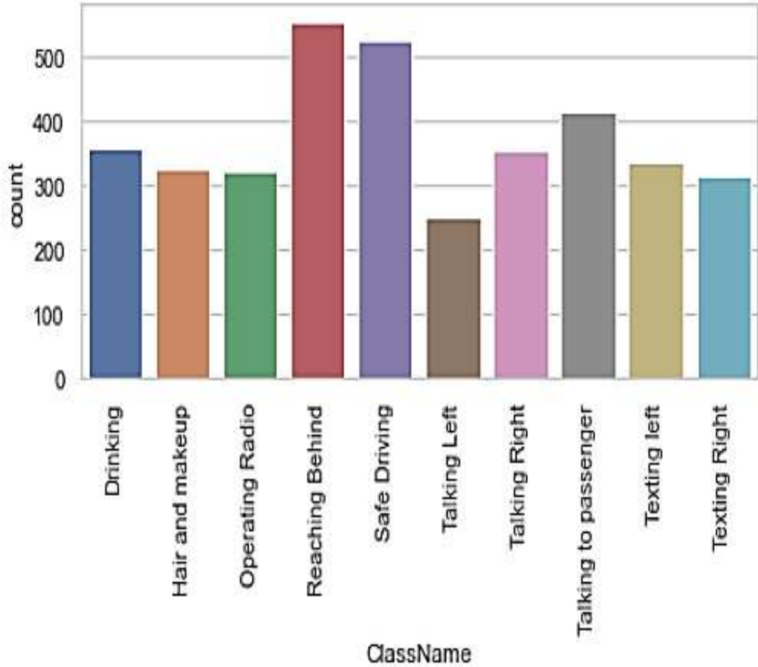
Figure 4 Statistic visualization of training data of our DDB Dataset.
