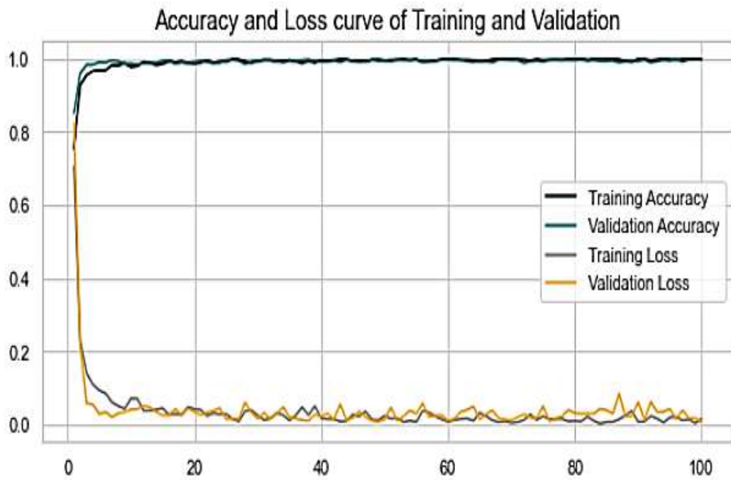
Figure 12 Accuracy and Loss curve of Adam Optimizer of our model in DDB Dataset
