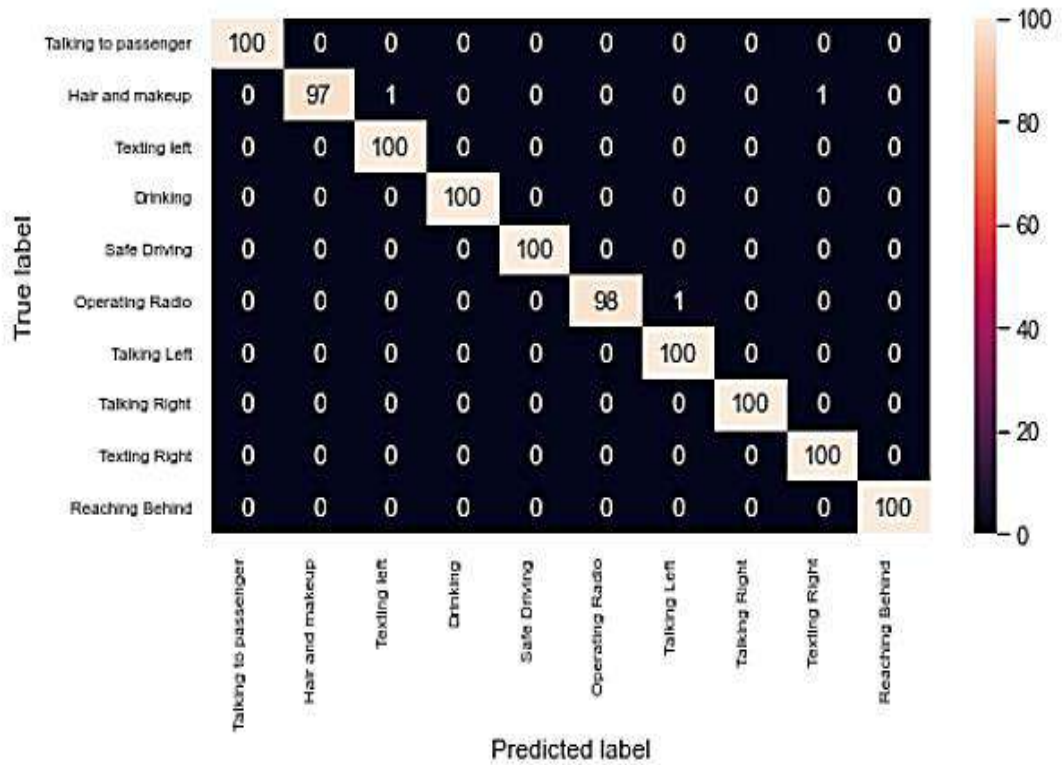
Figure 15 Confusion Matrix of SGD Optimizer in DDB Dataset
