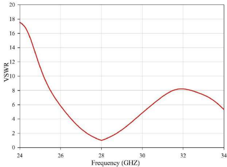
Figure 4.3: VSWR of Microstrip Patch Antenna
