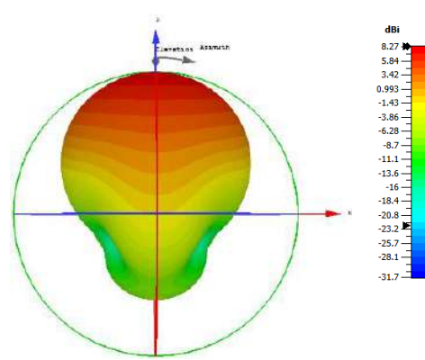
Figure 4.6: Microstrip Patch Antenna Directivity
