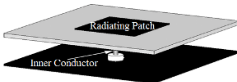
Figure 1.11: Coaxial probe feed [18]
