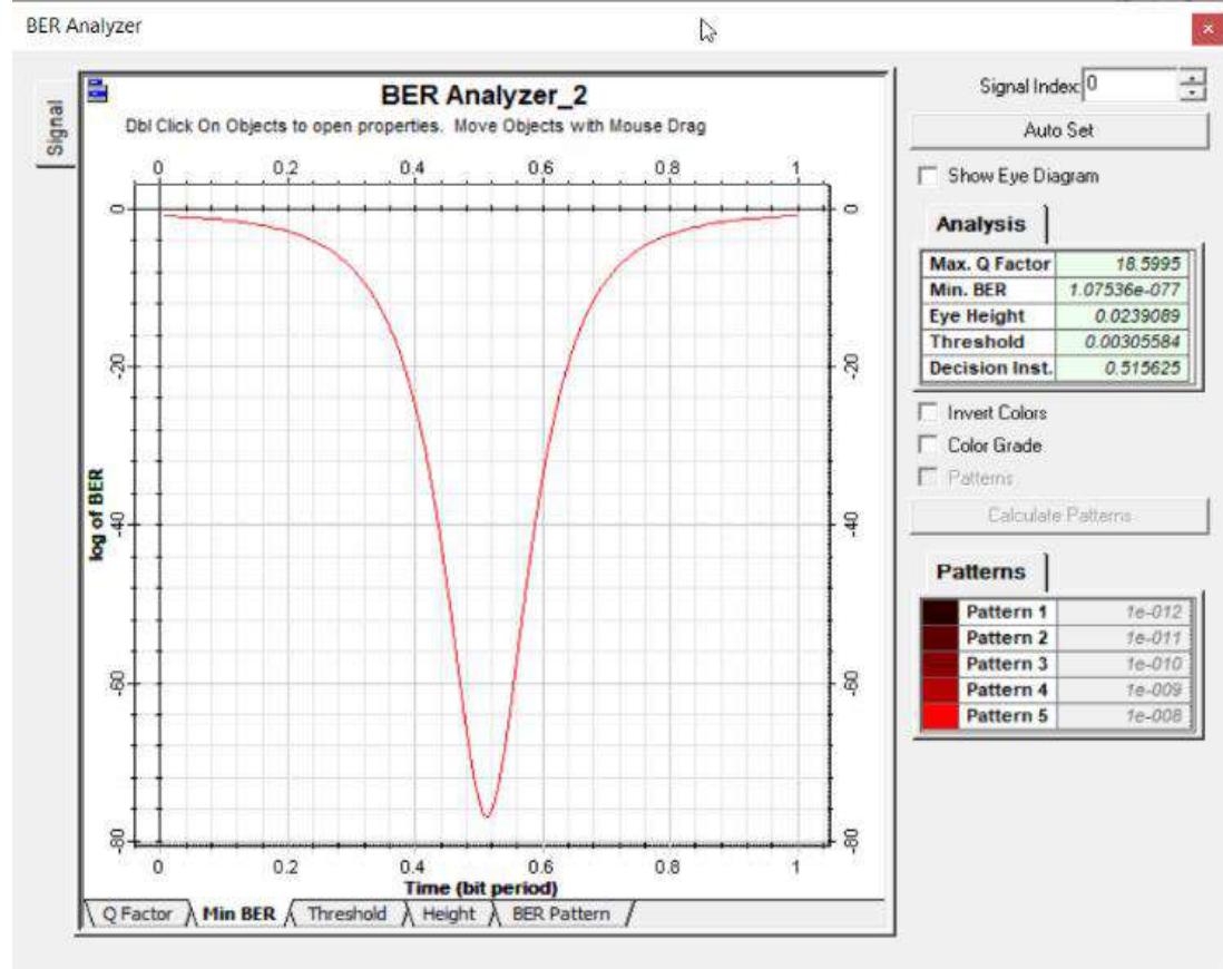
Figure 4.9 Bit Error Rate for Four Channel Environments
