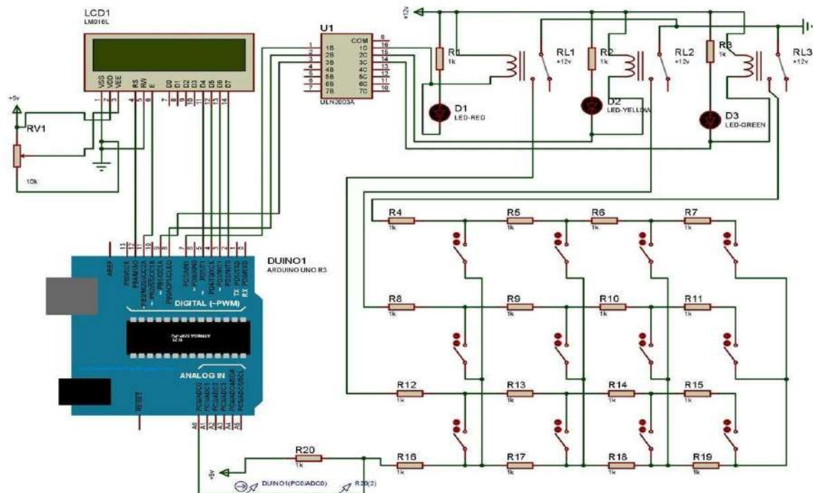
Fig 5.1: Underground fault detection system circuit diagram [10]
